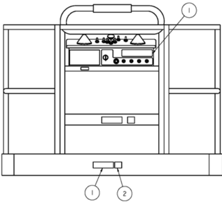
DECAL INSTALLATION AT PLATFORM TB42J/47J, TB66J, AB60J, TB80/85J, AB80J/85RJ
