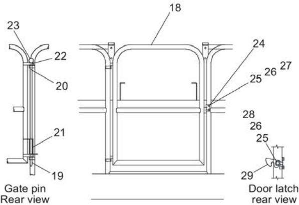
Swinging gate, aluminum platform
