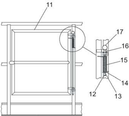
Swinging gate, steel platform
