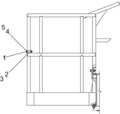
Gravity gate, steel platform
