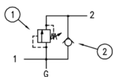
HYDRAULIC SCHEMATIC
