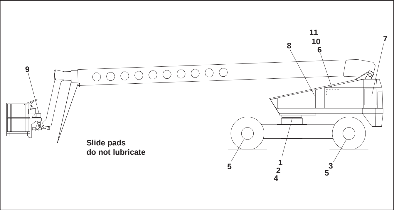
The illustration locates the lubrication points of the TB100J.
