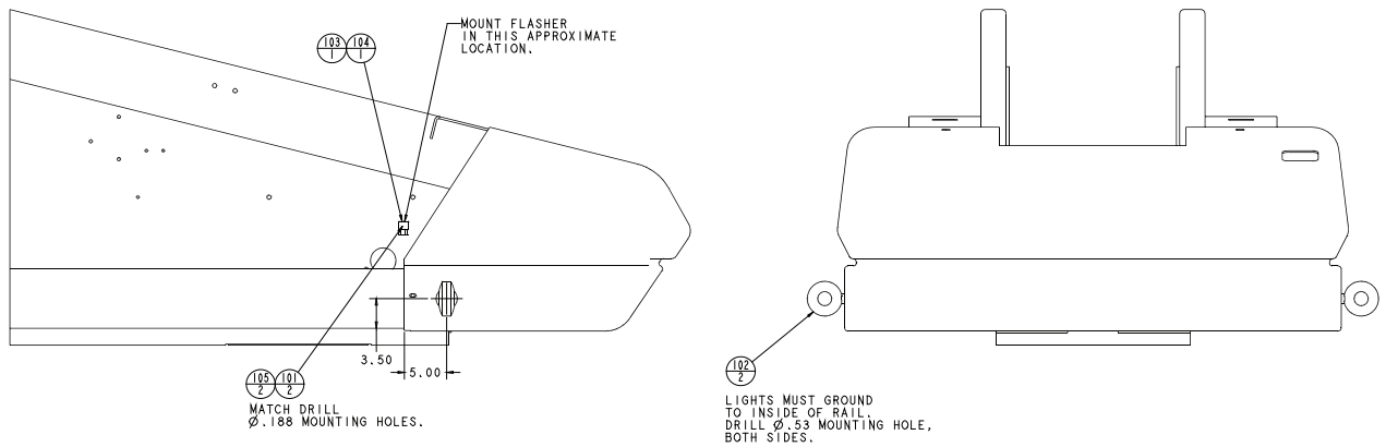
TAILLIGHT INSTALLATION
