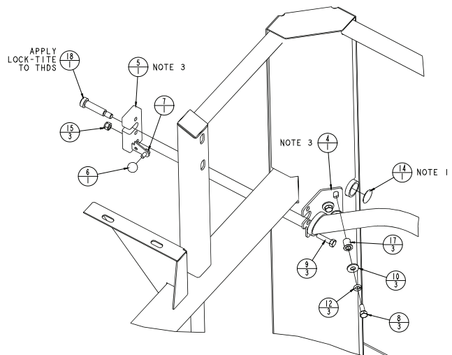
LATCH INSTALLATION
