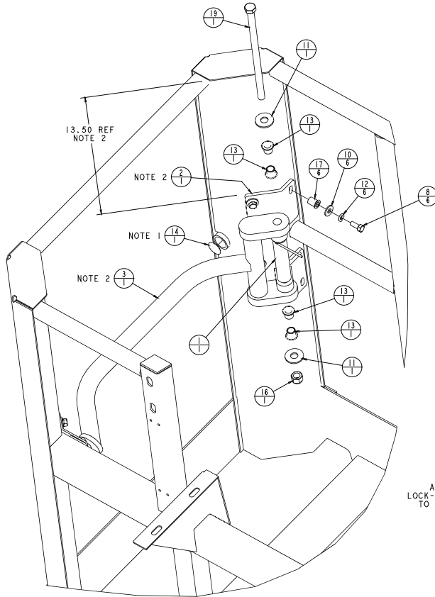
HINGE INSTALLATION
