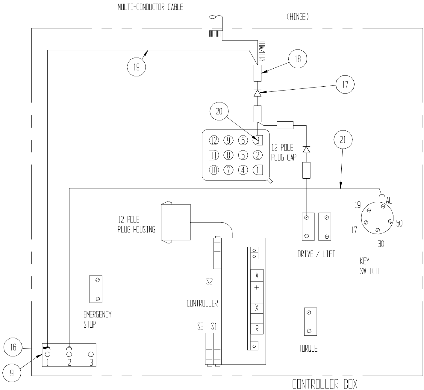
WIRING DIAGRAM
